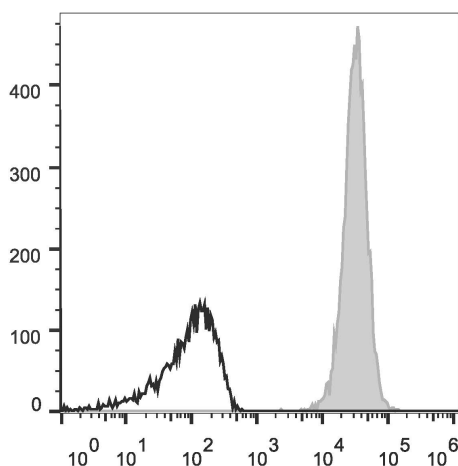
C57BL/6 murine splenocytes are stained with APC Anti-Human/Mouse/Rat CD47 Antibody (filled gray histogram). Unstained splenocytes (empty black histogram) are used as control.
