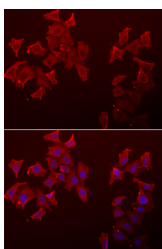
Immunofluorescence analysis of A549 cells using LECT1 Polyclonal Antibody
